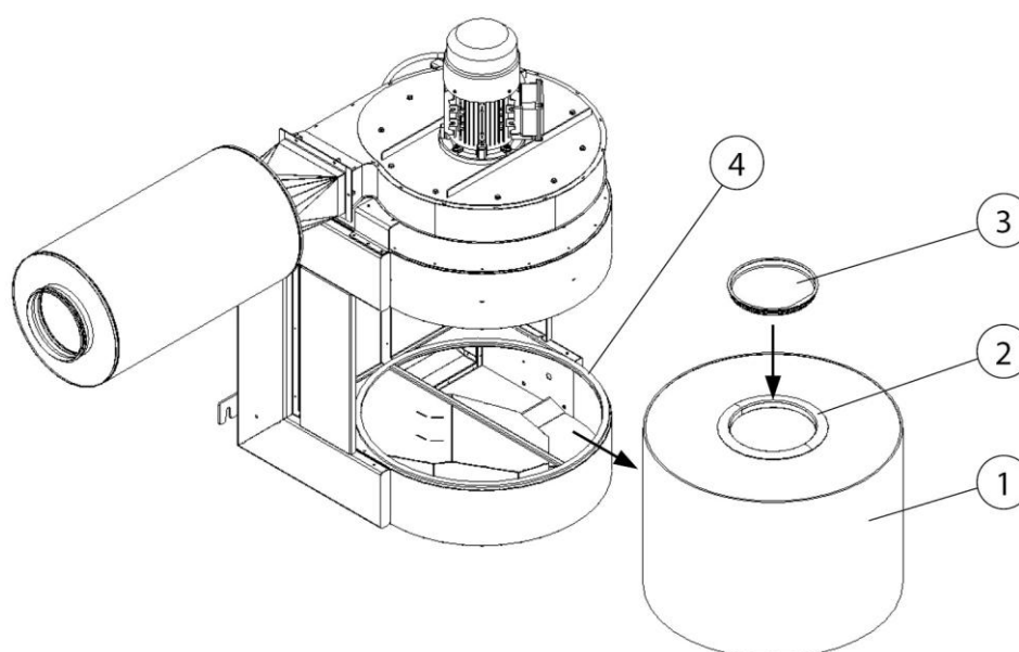
Fig. 14: Carrying out a filter change
