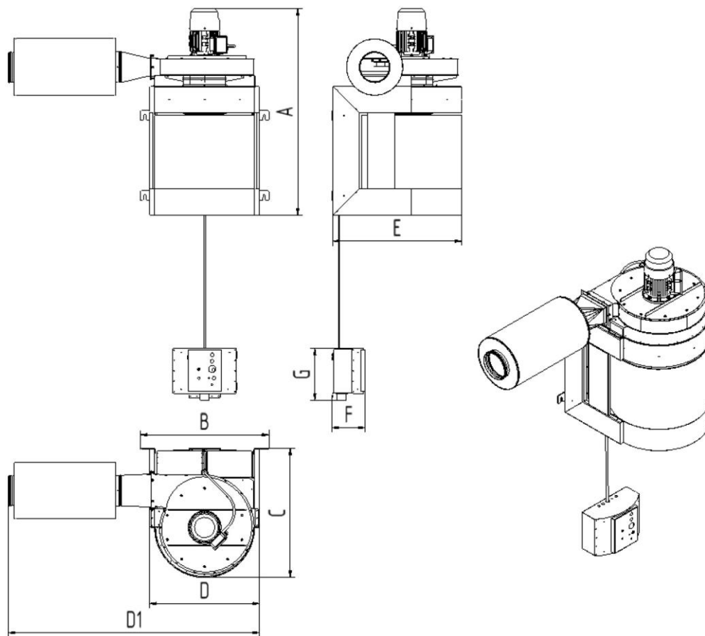
Fig. 17: Dimensions sheet
