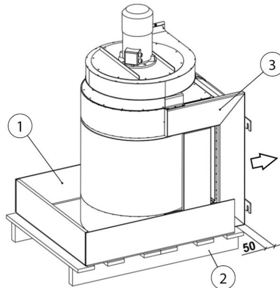
Fig. 4: Installation of the product
