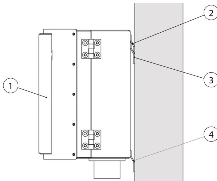
Fig. 8: Mounting the control box
