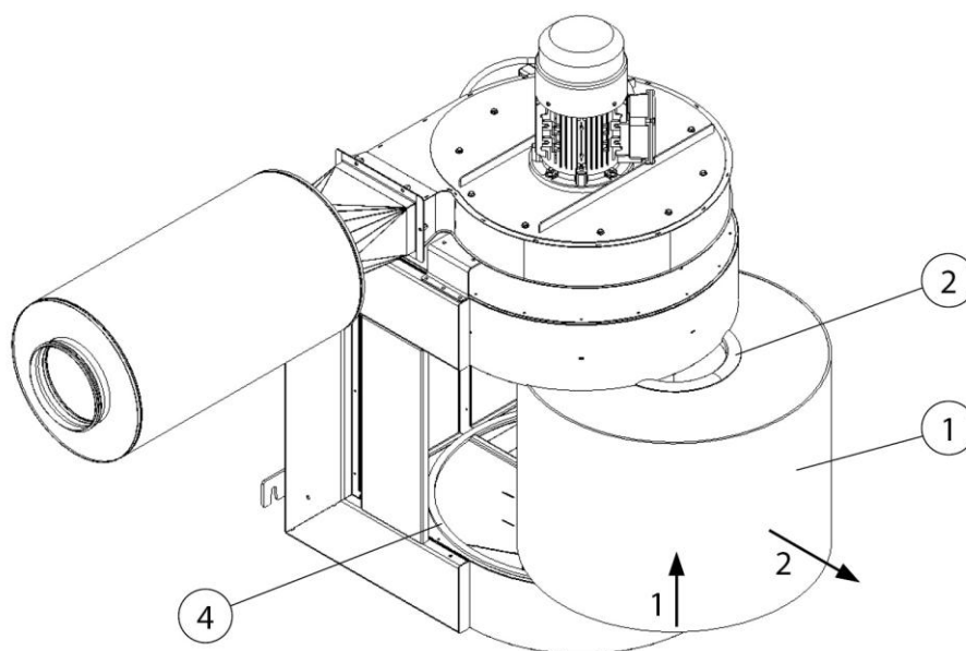
Fig. 13: Carrying out a filter change
