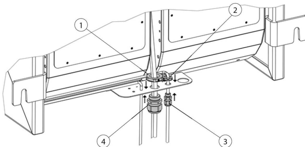
Fig. 5: Attaching the cable glands
